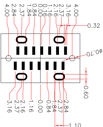
RECOMMENDED P.C.B. LAYOUT (T:1.00mm) TOLERANCE UNSPECIFIED ±0.05mm
