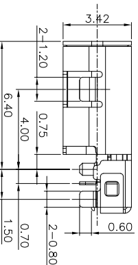
SECTION B-B
