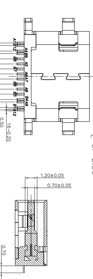
SECTION B-B SCALE 1:1
