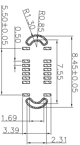
RECOMMENDED P.C.B. LAYOUT TOLERANCE UNSPECIFIED \pm 0.05\text{mm}
