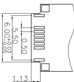
RECOMMENDED P.C.B. LAYOUT TOLERANCE UNSPECIFIED \pm 0.05\text{mm}
