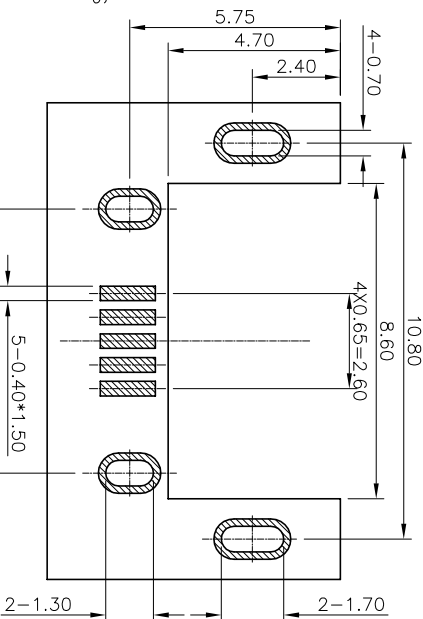
RECOMMENDED PCB LAYOUT TOP VIEW (Tol:±0.05)
