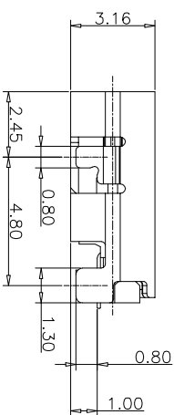
RECOMMEND P.C.B LAYOUT (COMPONENT SIDE) TOLERANCE FOR PCB LAYOUT IS ±0.05
