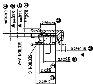
SECTION C Scale 5:1
