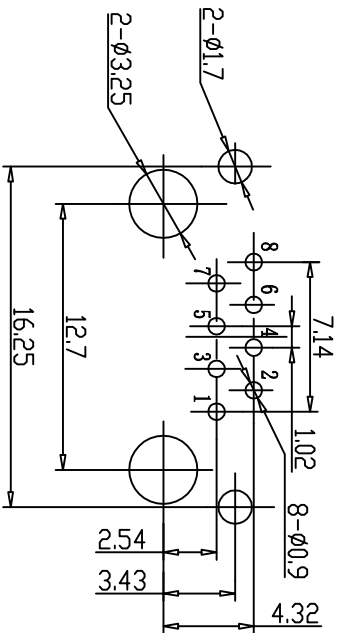
PC Board Layout
