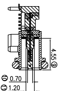
SECTION B-B SCALE 1/4"
