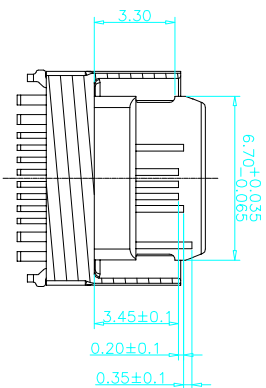
SECTION B-B SCALE 1:1
