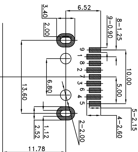
RECOMMENDED P.C.B LAYOUT TOLERANCES: ±0.05mm
