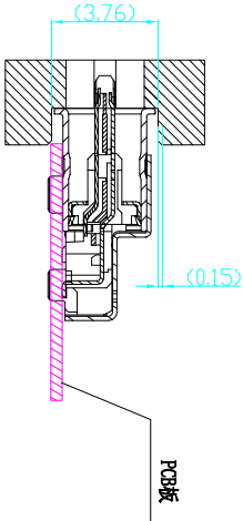
SECTION A-A PANEL CUT-OUT REFERENCE
