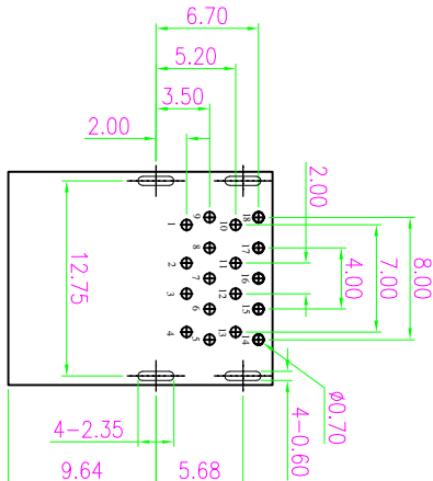
RECOMMENDED P.C.B HOLE LAYOUT TOP VIEW(TOLERANCE:±0.05)
