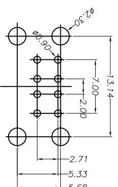
RECOMMENDED PCBA LAYOUT Top VIEW (TOLERANCE+±0.05)
